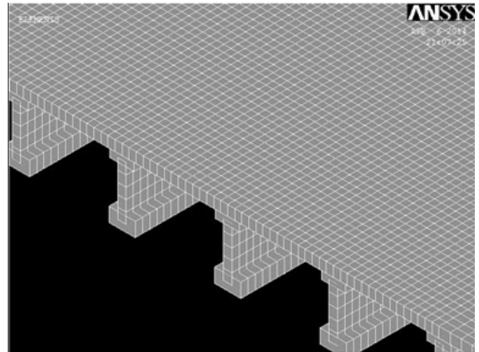
Mesh geometry of the bridge deck modeled by the FEM
