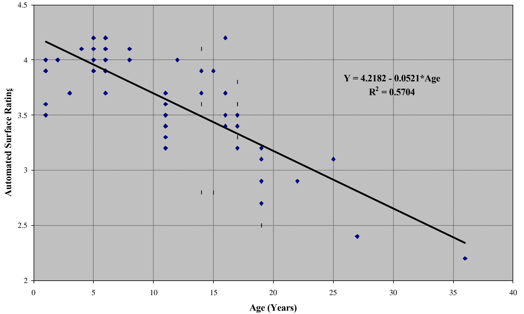
Figure 7. Asphalt Pavement Surface Rating Performance Model
