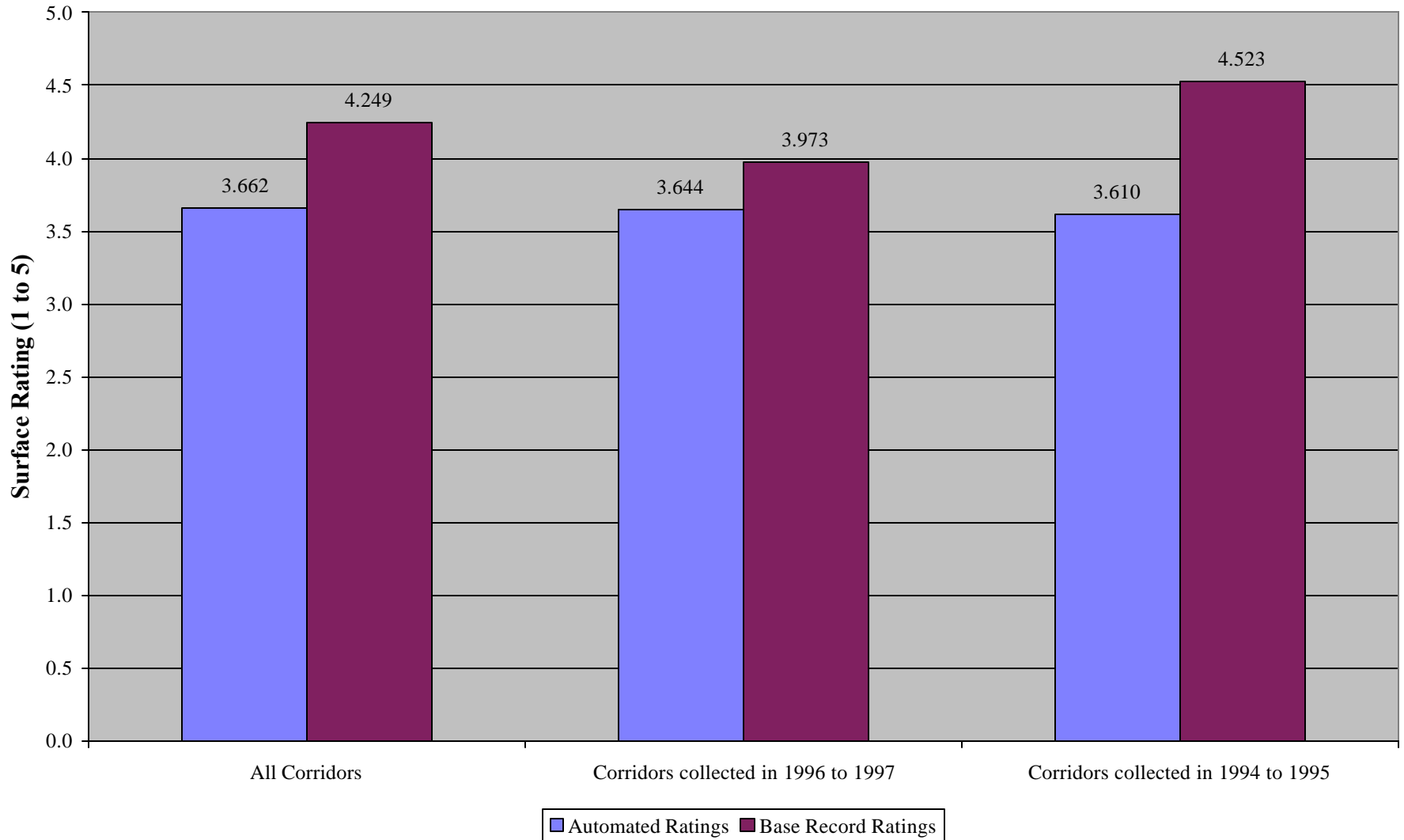
Figure 17. Original BR and AUTO Surface Ratings Comparisons
