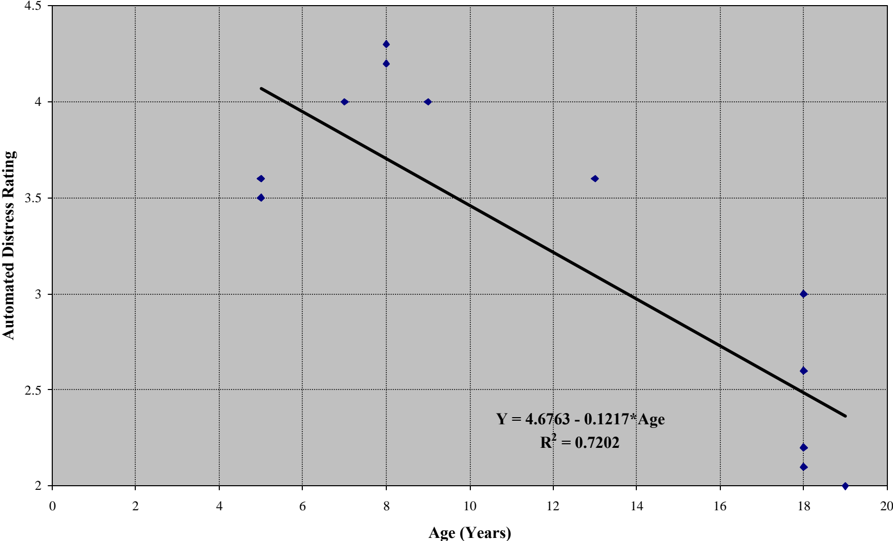
Figure 9. Composite Pavement Surface Rating Performance Model
