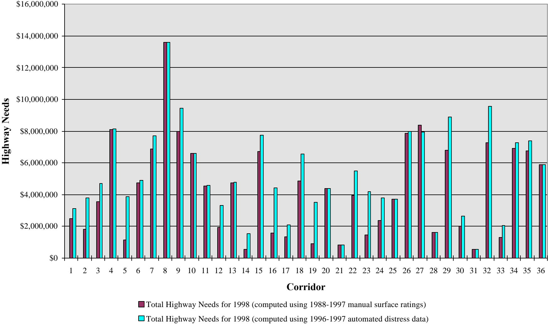
Figure 10. Base Record Ratings vs. Automated Distress Ratings (Needs Changes)
