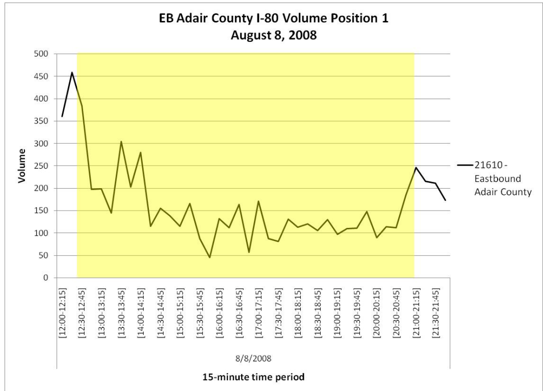
Figure 17. Traffic volume EB Adair County on August 8 during congestion period
