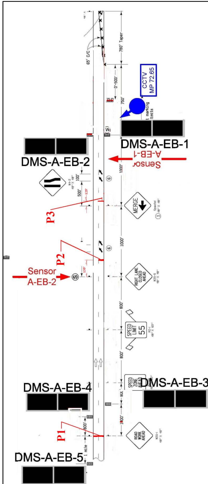
Figure 6. P1, P2, and P3 positions relative to static TTC and DMS signs
