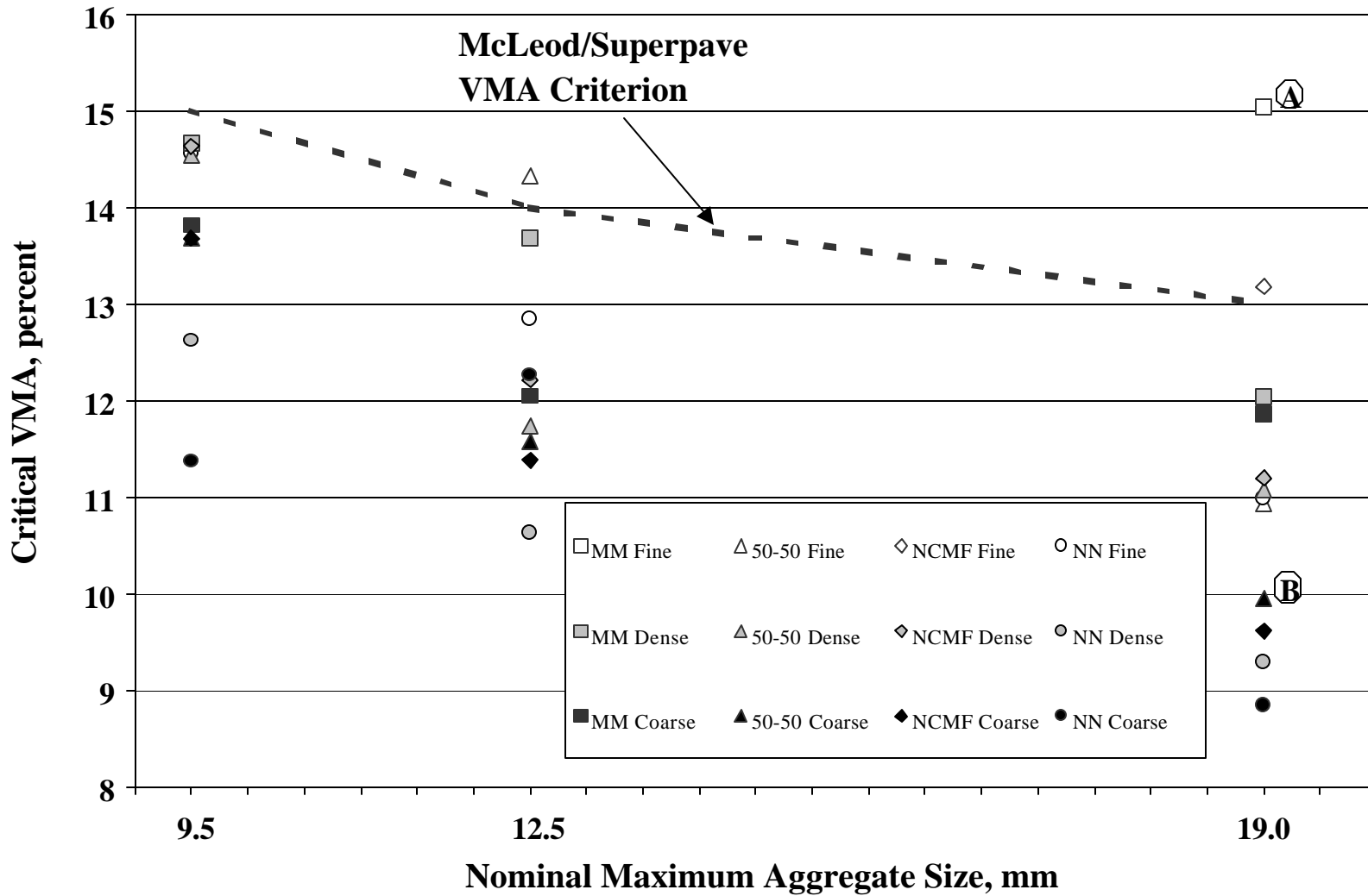
FIGURE 13 Observed Versus McLeod/Superpave Critical VMA
