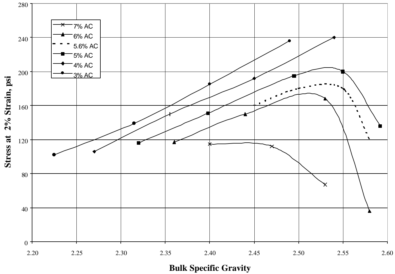
FIGURE 3 Stress at Two Percent Strain Versus Bulk Specific Gravity (1)
