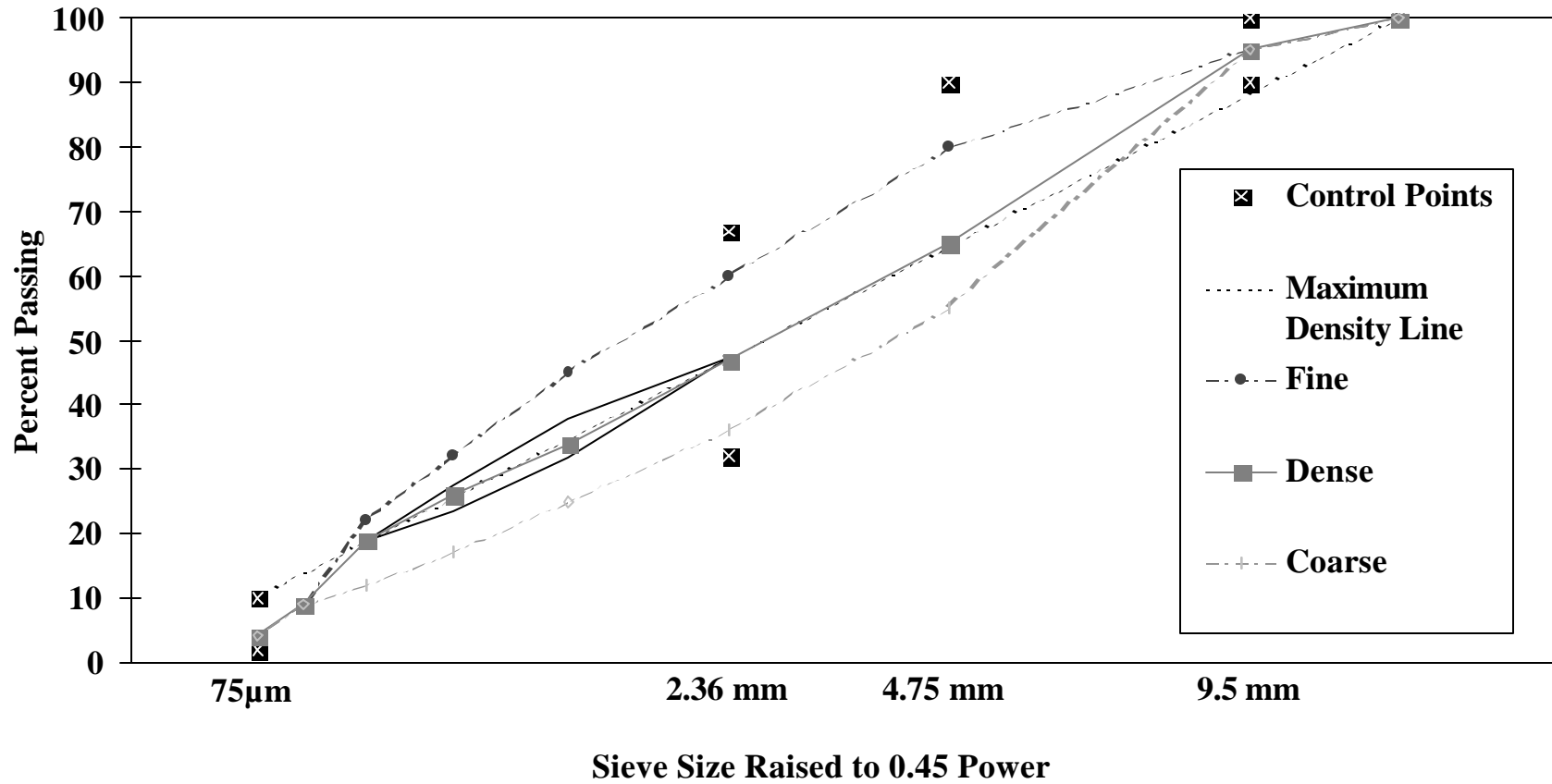
FIGURE 7 9.5-millimeter Nominal Maximum Size Gradations Used in Study
