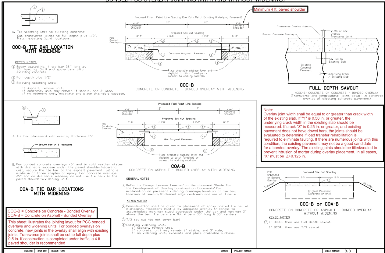
Figure 7.8. Widening details for COC-B and COA-B overlays
