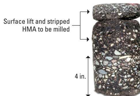
Figure 8.2. Core showing pavement that can be milled to remove stripped/unsound material, with 4 in. of HMA remaining in good condition
