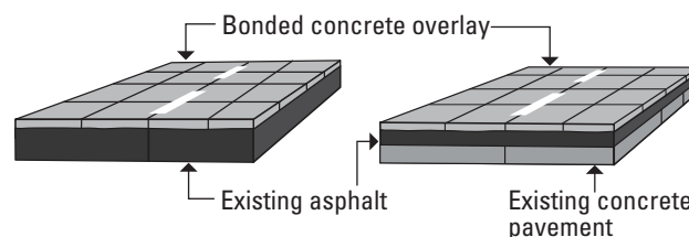
Figure 4.5. COA–B overlays on existing asphalt (left) and composite (right) pavements
