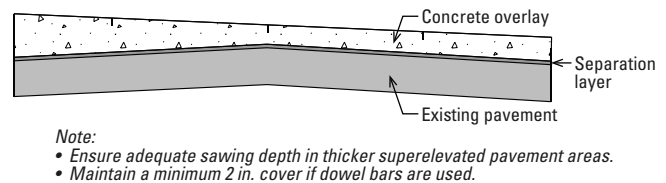
Figure 7.17. Superelevation detail
