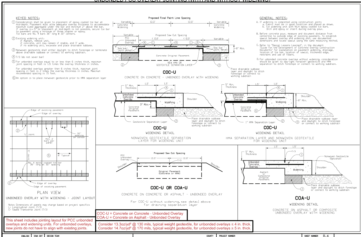
Figure 7.9. Widening details for COC-U and COA-U overlays
