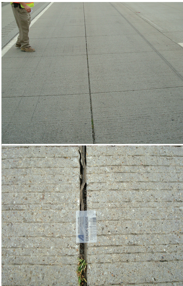
Figure A.5. COA-B overlay with tied lane joints and untied mid-lane longitudinal joint after eight years of service
