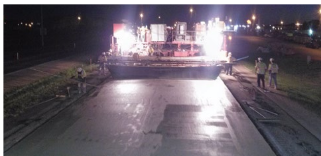
Figure 37. Nighttime paving on the West Dakota Parkway to avoid heavy traffic and allow for consistent delivery of mixture to the paver
