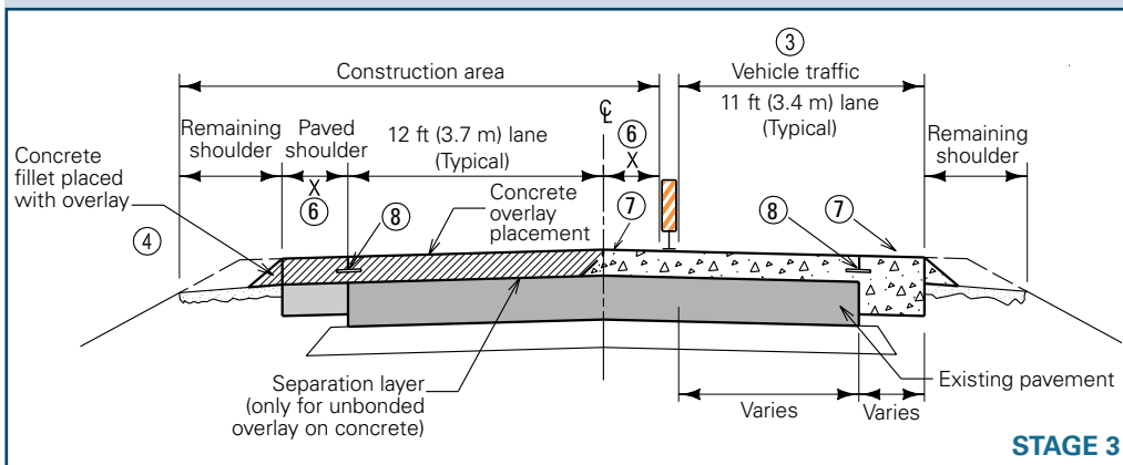
Figure 10. Example staging sequence diagram for two-lane roadway maintaining traffic
