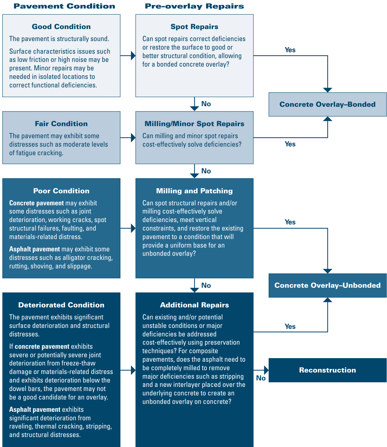
Figure 4. Decision tree for selecting the appropriate concrete overlay solution for a given project
