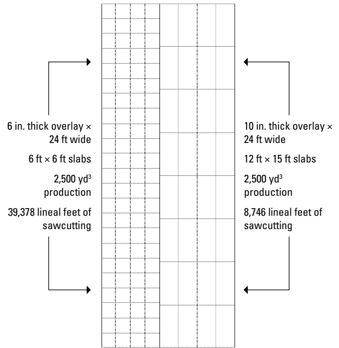
Figure 13. Comparison of sawcut lengths required for thinner (left) and thicker (right) overlays
