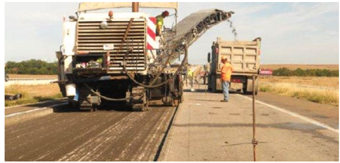
Figure 22. Profile milling of the existing pavement on I-70 using string line machine control
