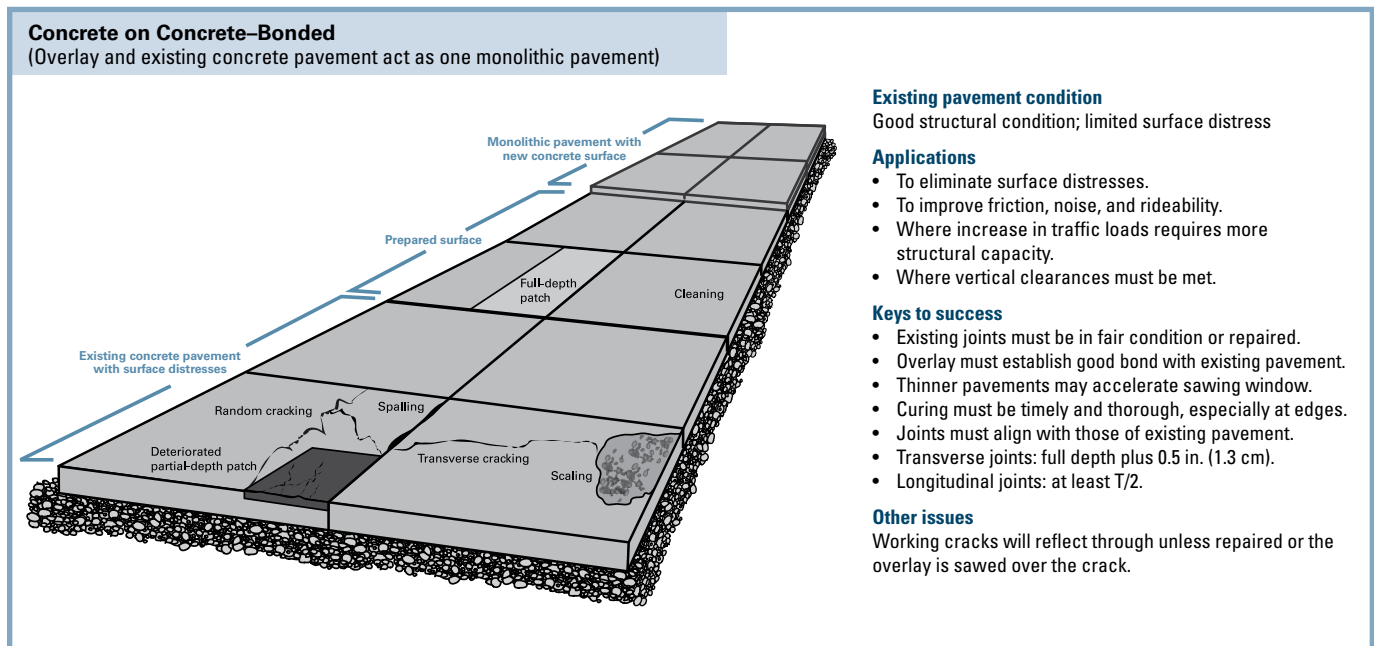
Figure 8. Summary of COC–B overlays
