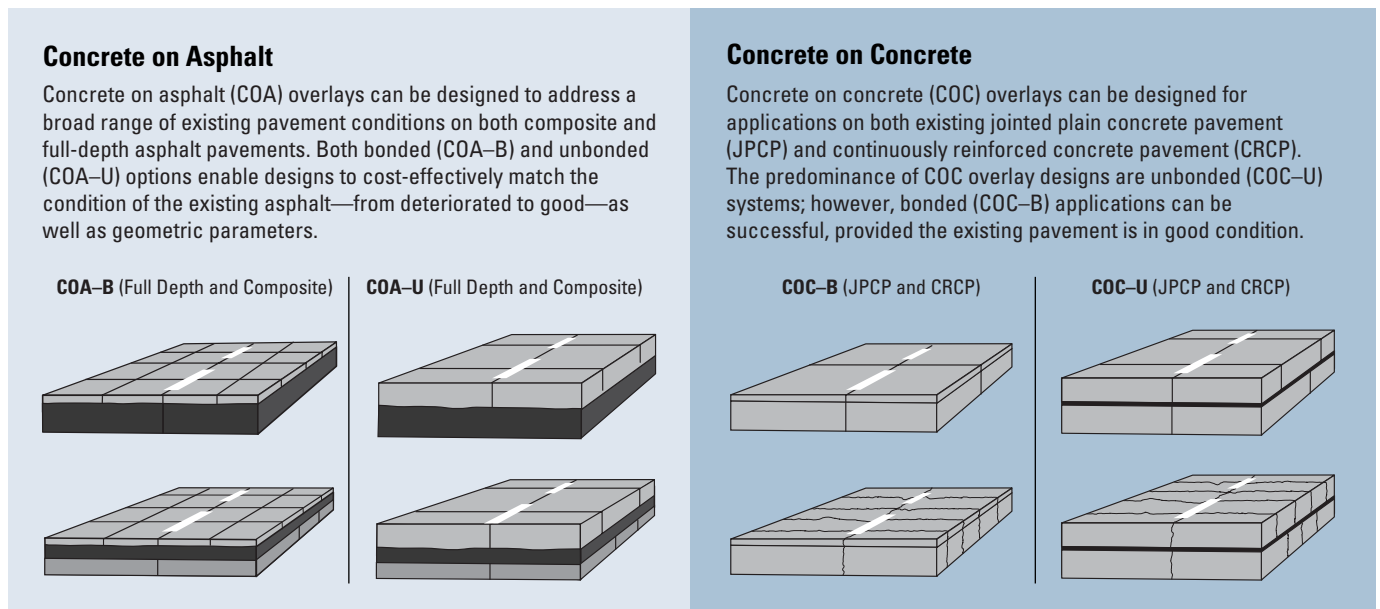
Figure 1. Summary of concrete overlay types on existing asphalt-surfaced and concrete pavements
