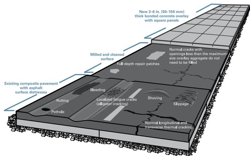
Figure 6. Summary of COA-B overlays
