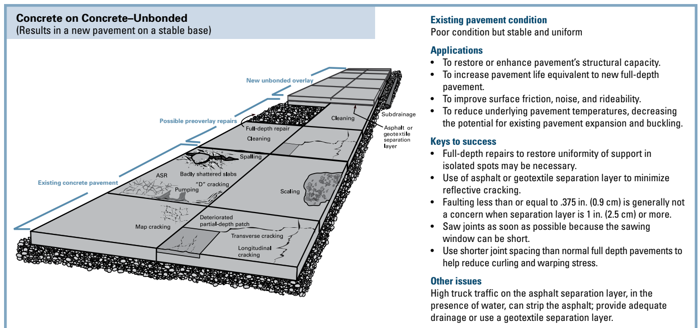
Figure 9. Summary of COC-U overlays
