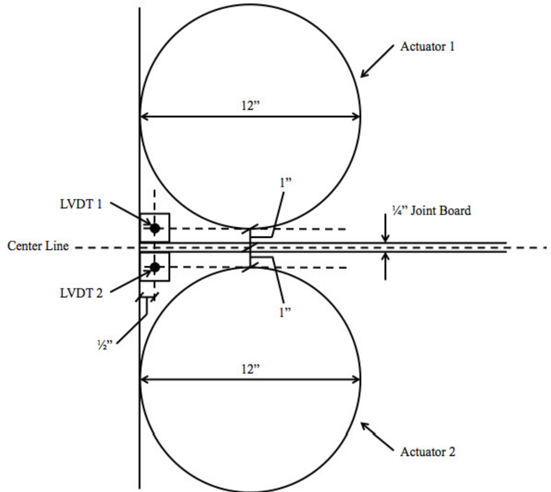
Figure 1. Schematic showing location of LVDTs relative to joint and actuator load plates (Source: J. Vandebossche, Univ. of Pittsburgh, 2017).
