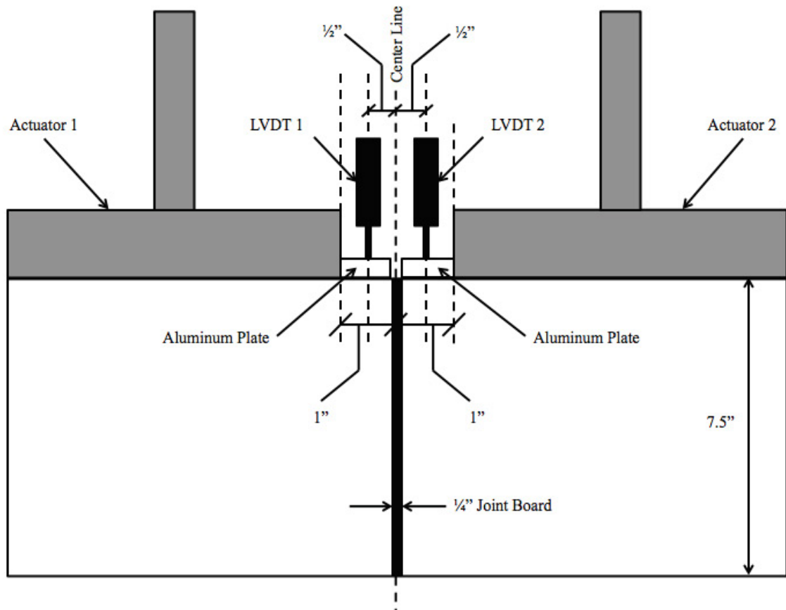
Figure 4. Schematic showing location of LVDTs relative to joint and actuator load plates (Source: J. Vandebossche, Univ. of Pittsburgh, 2017).
