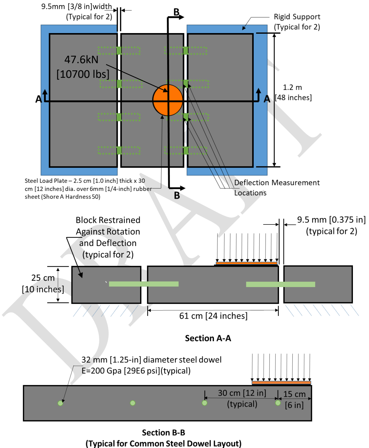
Figure 1. Load-Deflection Test Schematic
