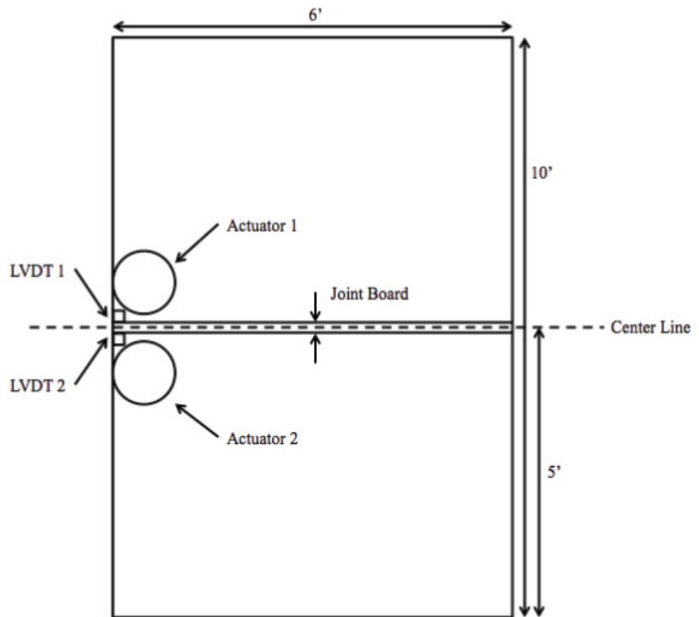
Figure 6. Schematic showing location of LVDTs relative to joint and actuator load plates (Source: J. Vandebossche, Univ. of Pittsburgh, 2017).
