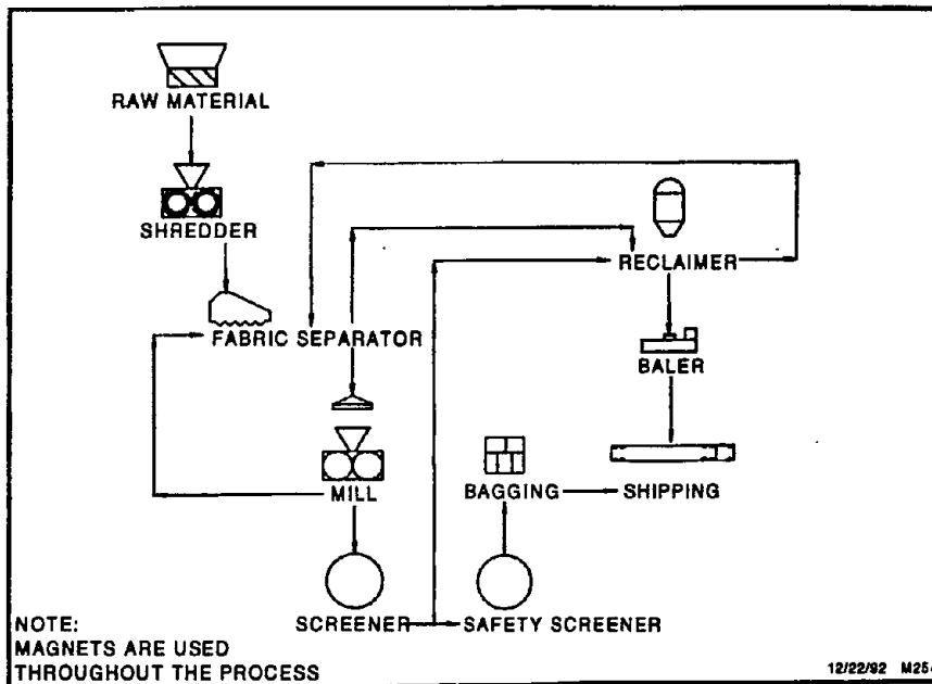
Figure 3-1. Basic ambient tire grinding process
