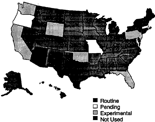
Figure 6-1d. Use of CRM in OGFC
