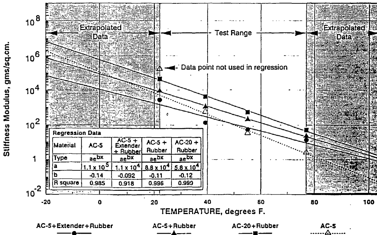
Figure 9-2. Stiffness Modulus vs. Temperature
