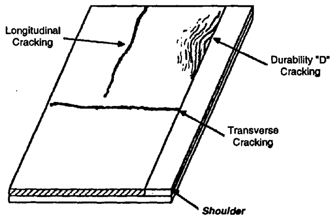
Figure 2-17. Cracking of continuously reinforced concrete pavement
