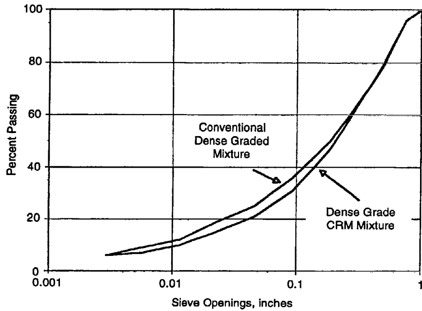
b) Dense-graded CRM
