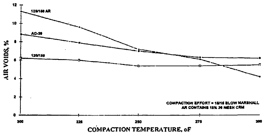
Figure 10-2. Air voids vs. compaction temperature for HMA with AC-20, 120/150, and AR
