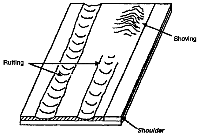
Figure 2-11. Surface deformation of asphalt concrete pavement
