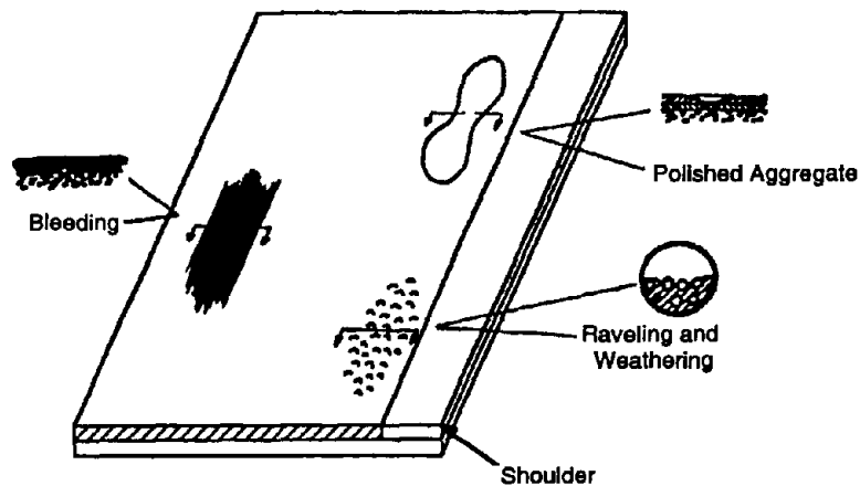
Figure 2-12. Surface defects of asphalt concrete pavement
