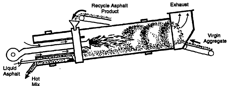
Figure 2-7. Counter flow drum mixer components (Astec)
