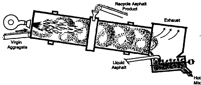
Figure 2-6. Drum mix coater cutaway (Astec)
