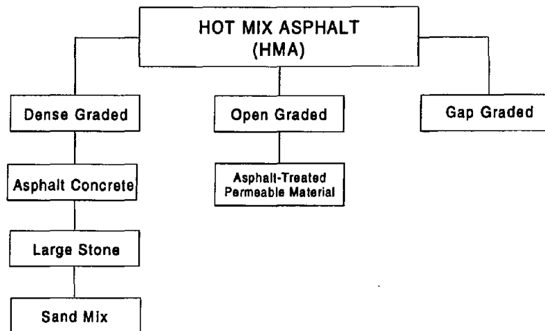
Figure 2-1. Types of HMA mixes
