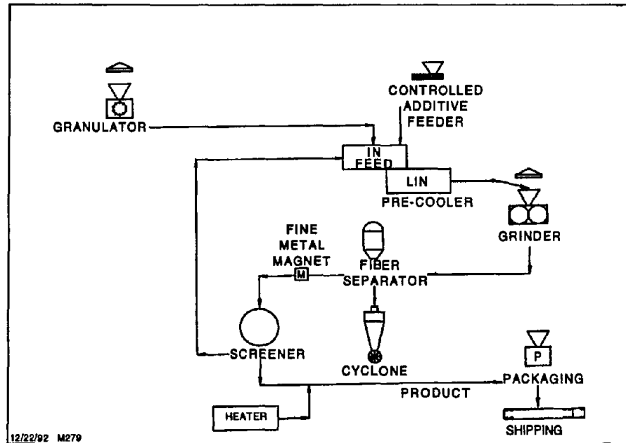
Figure 3-2. Basic cryo grinding system
