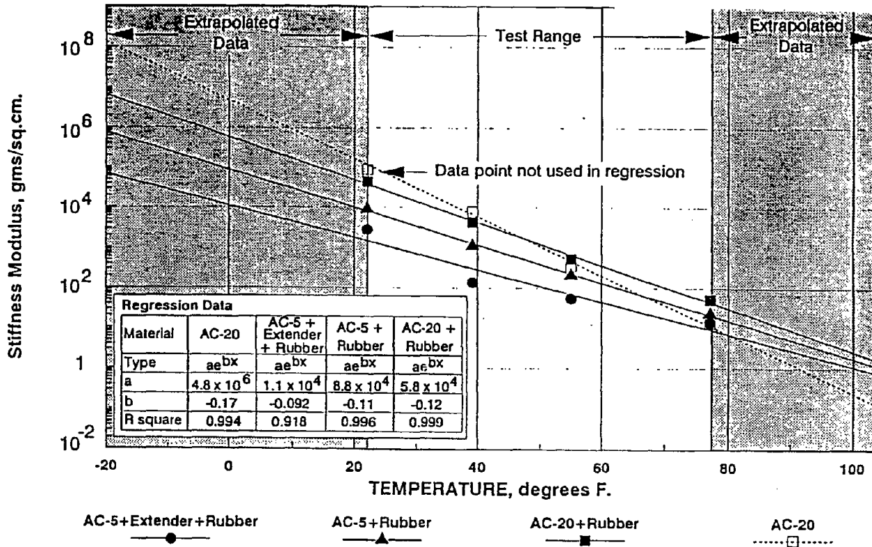
Figure 9-4. Stiffness Modulus vs. Temperature
