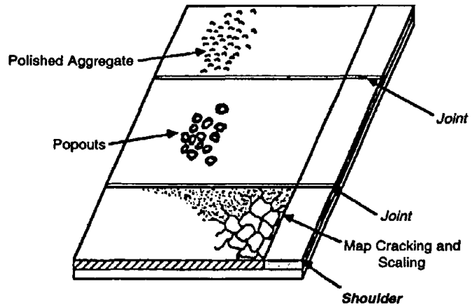
Figure 2-15. Surface defects of jointed concrete pavement.
