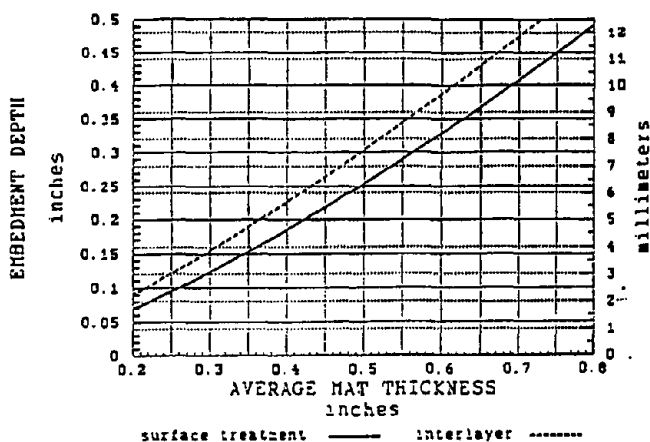
Figure 10-5. Embedment depth factors for AR surface treatment design 1
