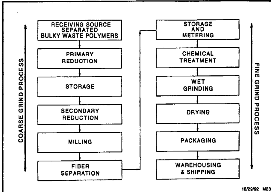
Figure 3-3. Basic wet grinding system
