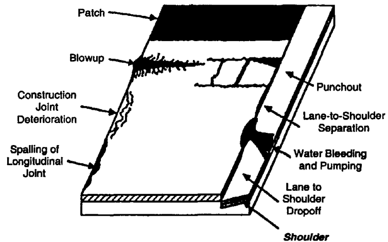
Figure 2-19. Miscellaneous defects of continuously reinforced concrete pavement
