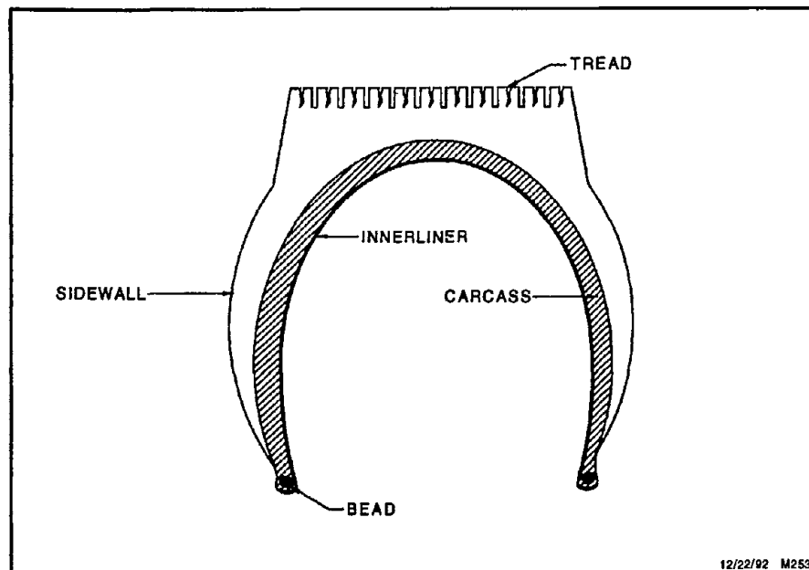
Figure 3-4. Typical tire cross-section
