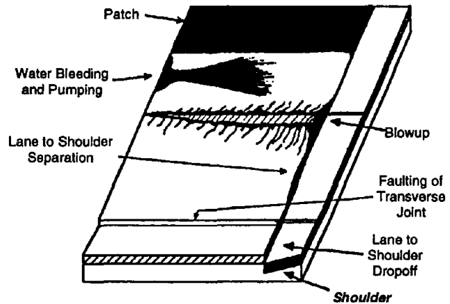
Figure 2-16. Miscellaneous distresses of jointed concrete pavement
