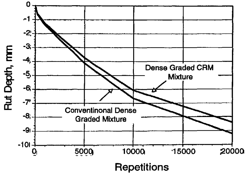
Figure 10-10. Rut resistance for RUMAC using LCPC wheel tracking device—dense-graded generic mix (after Lundy et al., 1992)
