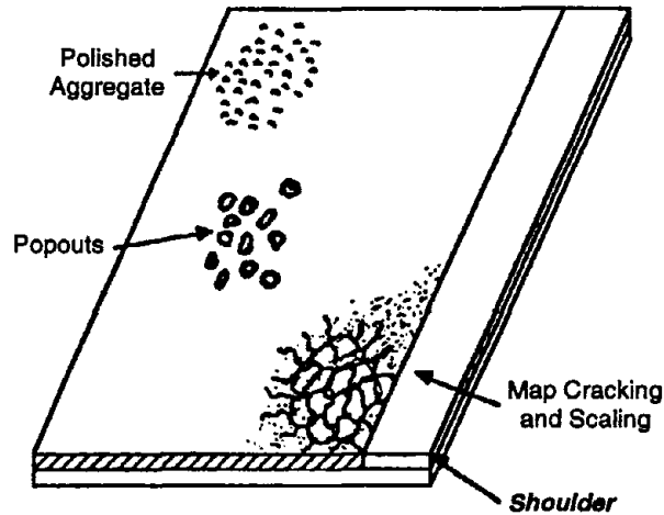
Figure 2-18. Surface defects of continuously reinforced concrete pavement
