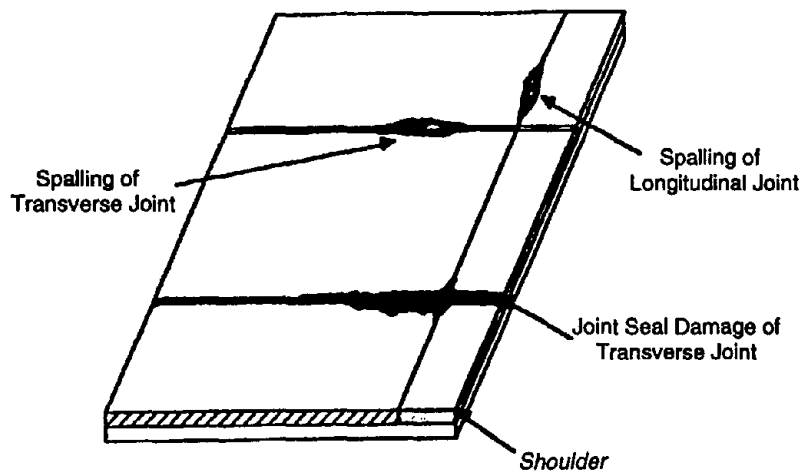
Figure 2-14. Joint deficiencies of jointed concrete pavement
