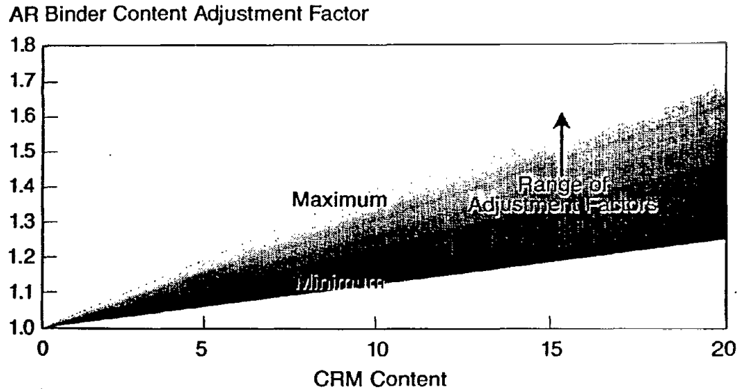
Figure 10-4. Open-graded AR mixture binder content adjustment factors
