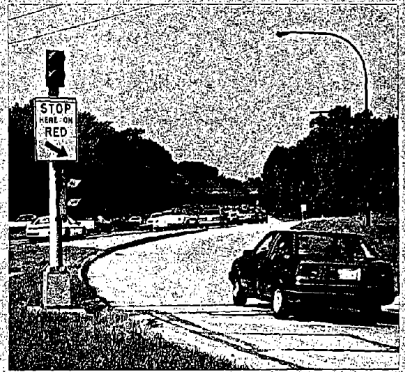
Computer-timed merge lights let vehicles enter one at a time to keep traffic moving more smoothly.
