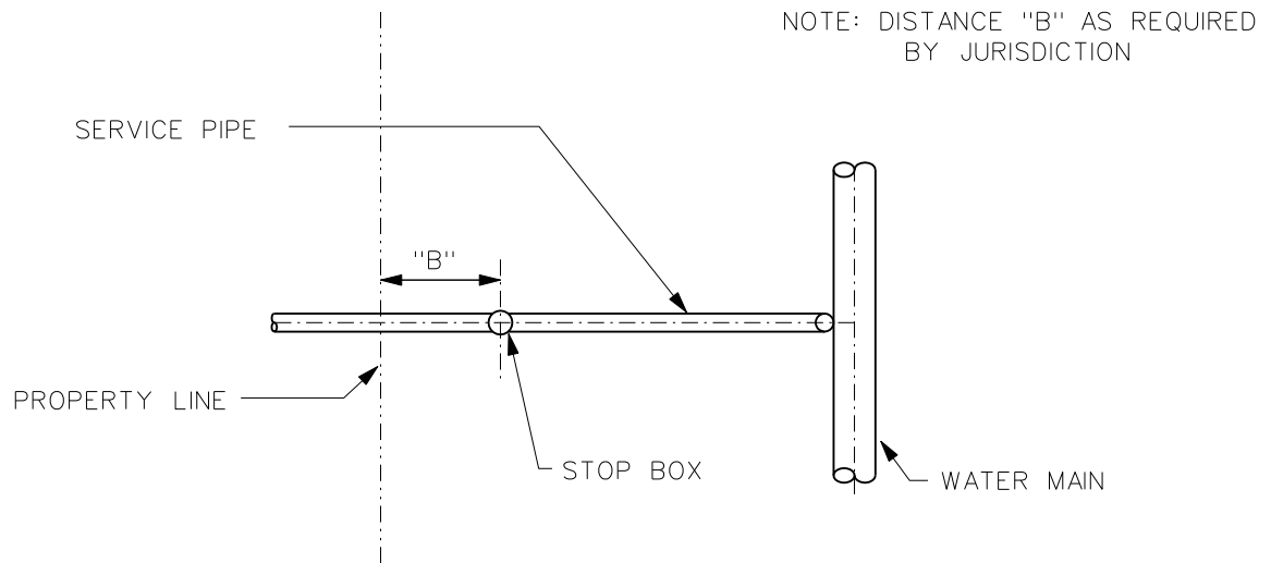
PLAN
