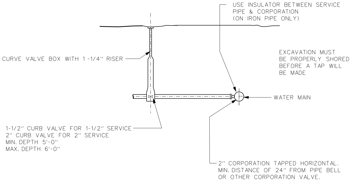
SECTION
