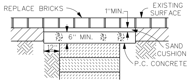
BRICK PAVEMENT
