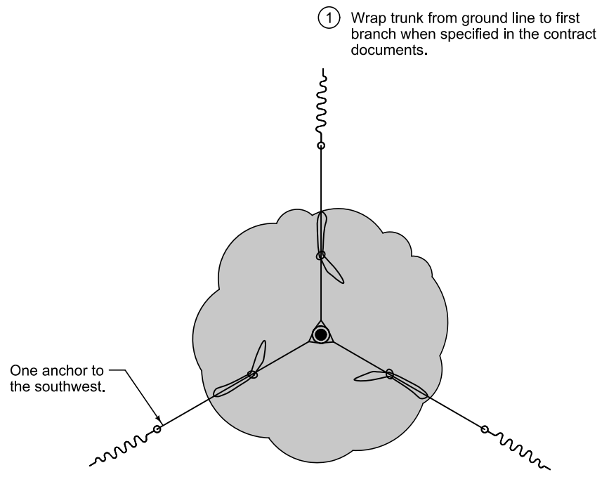
GUYING PLAN
