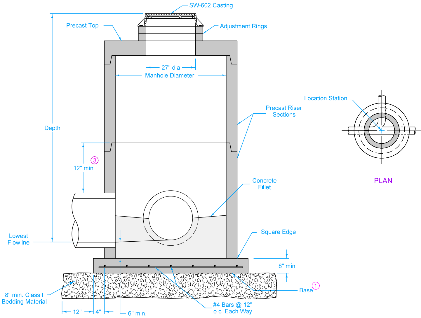
TYPICAL SECTION
