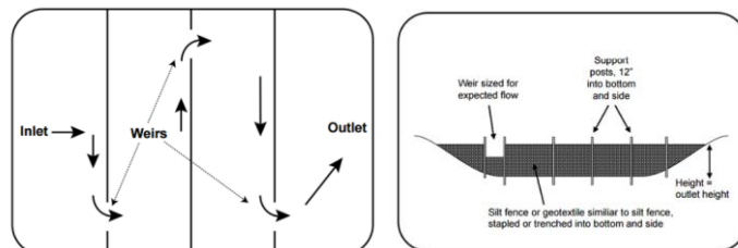
Figure 7E-12.05: Solid Baffles to Lengthen Flow Path
