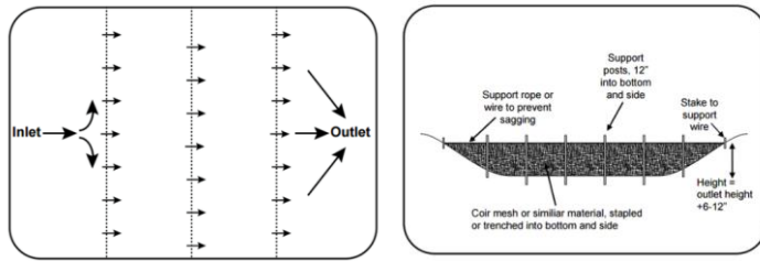
Figure 7E-12.06: Porous Baffles Develop Uniform Flow
