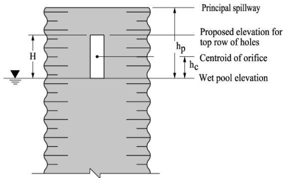
Figure 7E-12.015: Theoretical Discharge Orifice for Design of Perforated Risers
