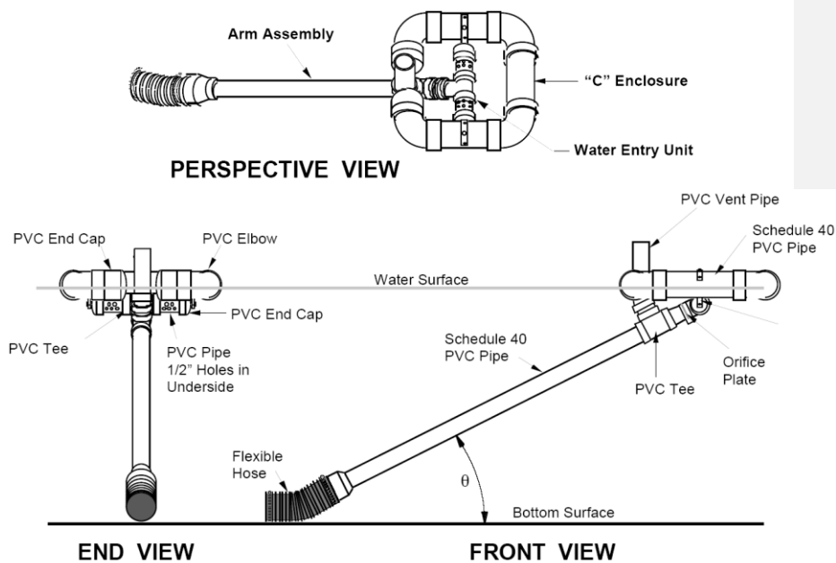
Figure 7E-12.062: Example Skimmer for Drawdown of Wet Storage
