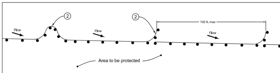
Figure 7E-14.02: Typical Silt Fence Installation for Perimeter Control
