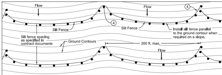
Figure 7E-14.01: Typical Silt Fence Installation for Slope Control
