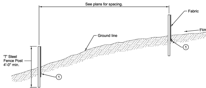
Figure 7E-14.01: Typical Ditch Check Spacing
