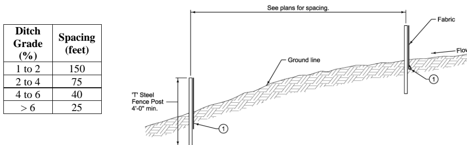
Figure 7E-14.01: Typical Ditch Check Spacing
