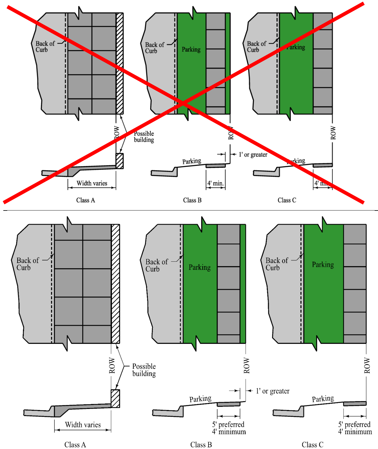
Figure 12A-1.01: Classes of Sidewalk
