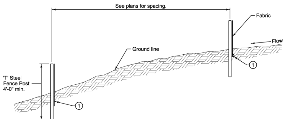
Figure 7E-14.01: Typical Ditch Check Spacing
