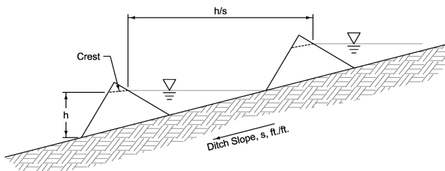
Figure 7E-7.01: Typical Check Dam Spacing (From SUDAS Specifications Figure 9040.106)
